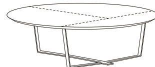
T51 MOON Ø100XH.32 / Ø39XH.13"
